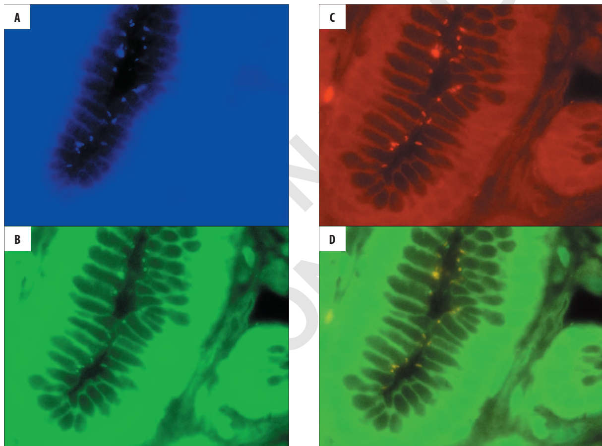
Figure 1. Visualization of H. pylori in gastric biopsy specimen by FISH. Panels A , B , C , and D demonstrate the same microscopic field under the relevant filter. (A) shows bacteria in blue because of staining DNA with DAPI. (B) demonstrate bacteria in green, indicating hybridization with probe Hpy-FLOUS. (C) shows red signal, indicating hybridization with probe ClAR1-Cy3, ClAR2-Cy3, or ClAR3-Cy3; therefore the strain is clarithromycin resistant. (D) the combination of red and green of a resistant strain represent a yellow or orange signal. The specimen contains a number of coccoid forms.
